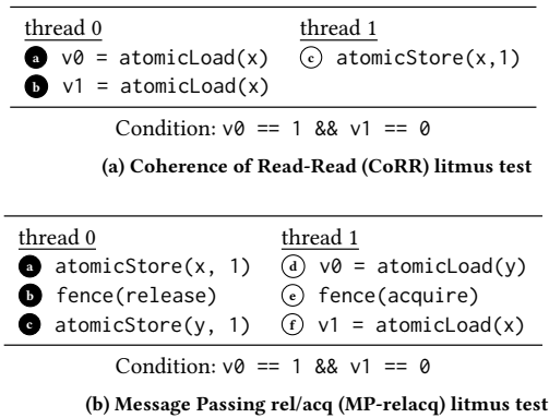
Figure 1: Two litmus tests that illustrate bugs in WebGPU found by our work. We observed executions that resulted in the condition being true, even though it is disallowed by the MCS. All memory is initialized to 0.
